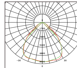
AVERAGE BEAM ANGLE (50%):91.4 DEG UNIT:cd — C0/180,93.0° — C90/270,89.8°
