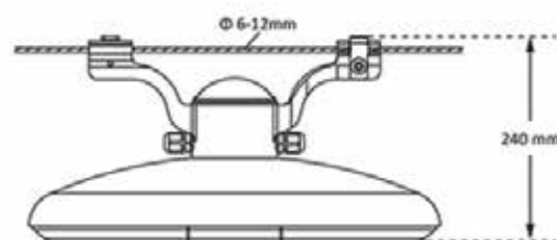
Suspended Mounted
