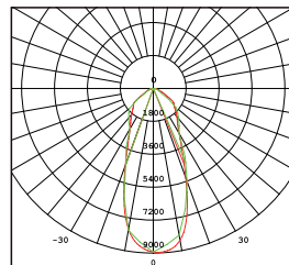
AVERAGE BEAM ANGLE (50%):42.9 DEG UNIT:cd — C0/180,42.1° — C90/270,43.6°
