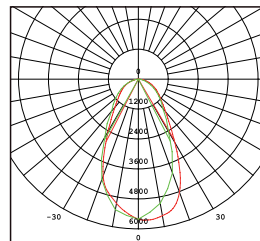
AVERAGE BEAM ANGLE (50%):57.3 DEG UNIT:cd — C0/180,57.9° — C90/270,56.6°
