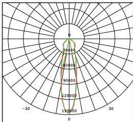
AVERAGE BEAM ANGLE (50%):24.0 DEG UNIT:cd — C0/180,23.9° — C90/270,24.2°
